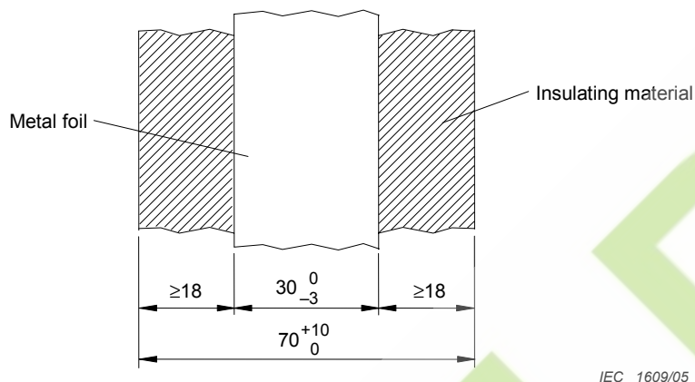
Figure AA.4 – Position of metal foil on insulating material
